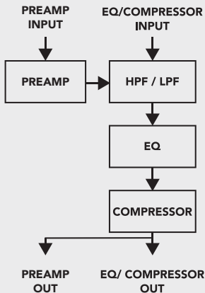
STANDARD MODE SIGNAL FLOW
